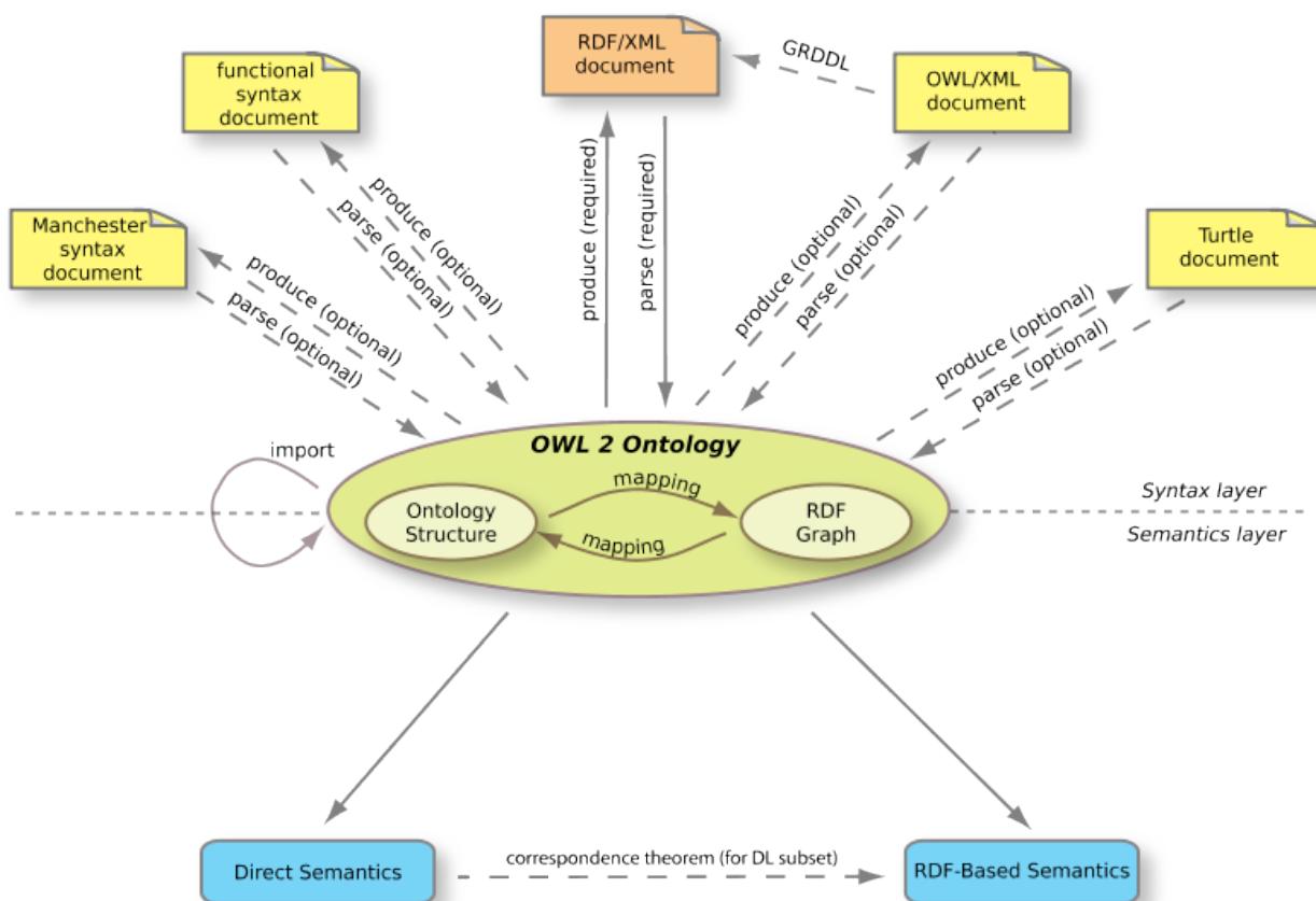
Figure 1. The Structure of OWL 2
